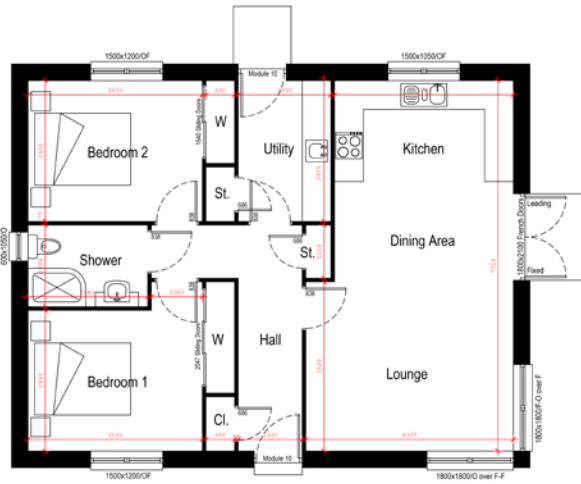
GROUND FLOOR PLAN Total Floor Area - 77.94m 2 (to plasterboard) Total Kit Area - 79.56m 2 (to structural kit)
