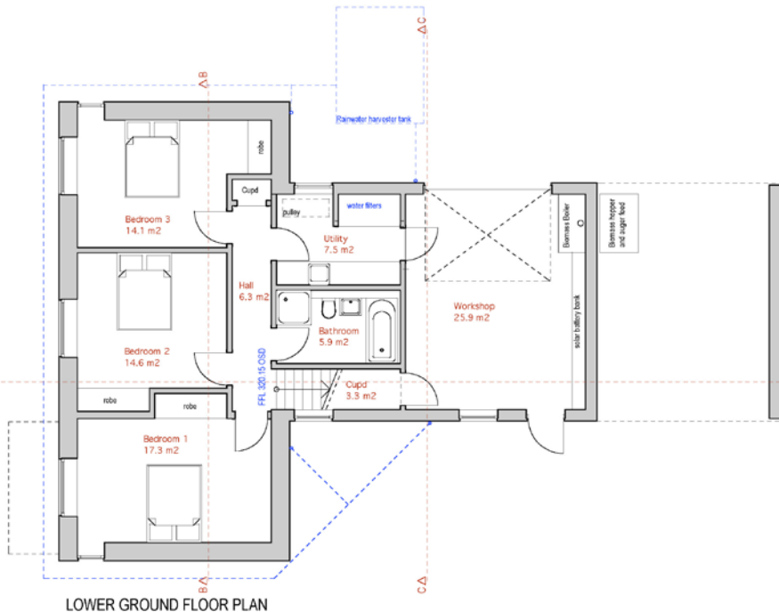
LOWER GROUND FLOOR PLAN
