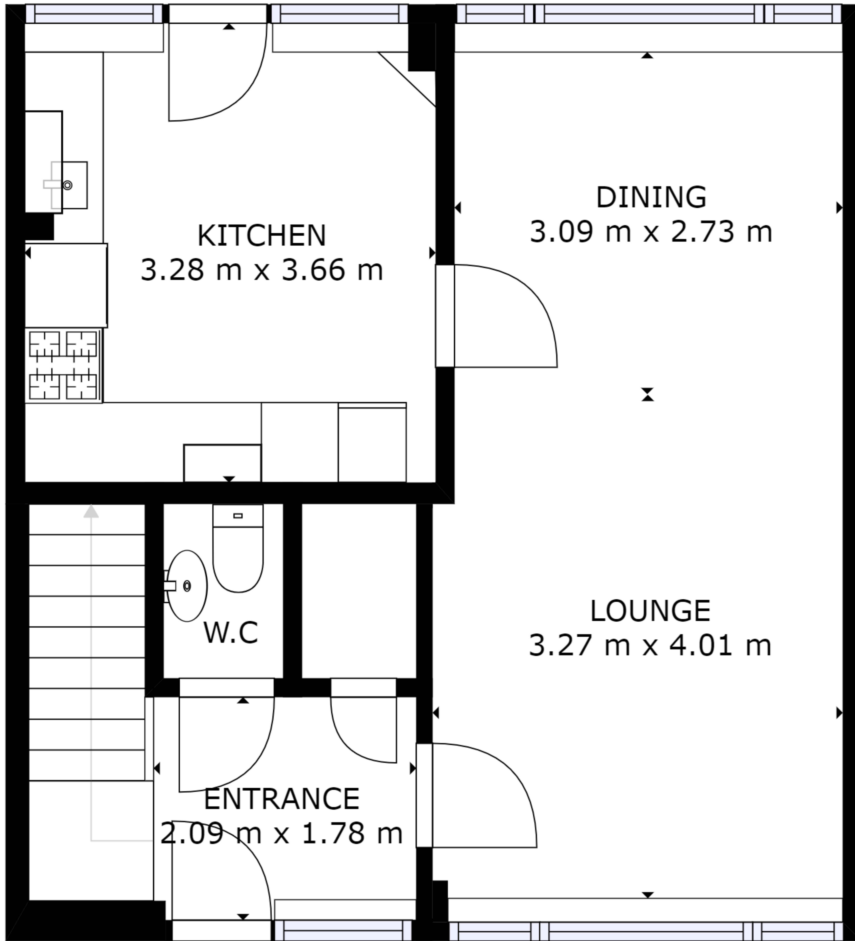
FLOOR 1
