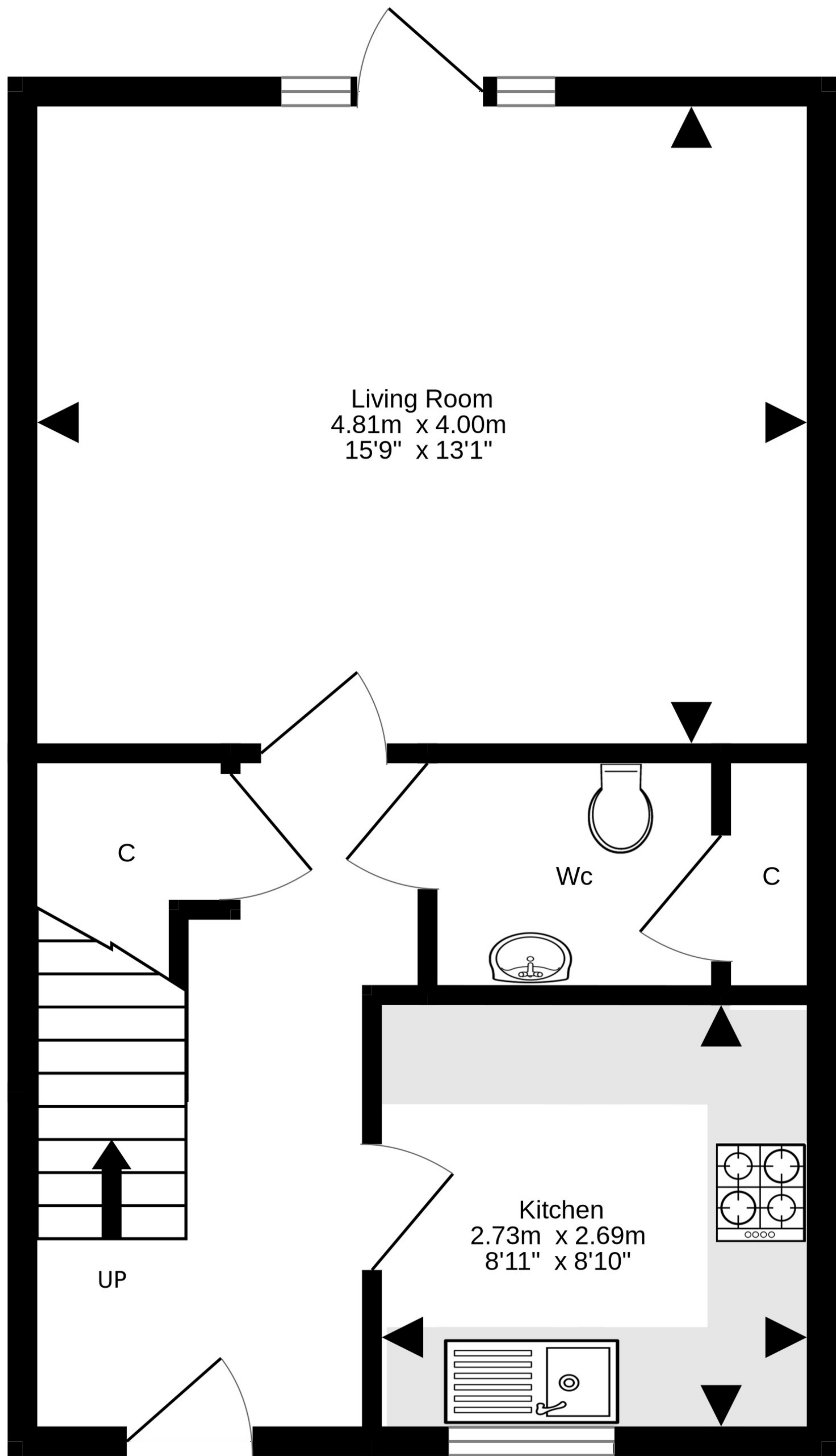
Ground Floor
