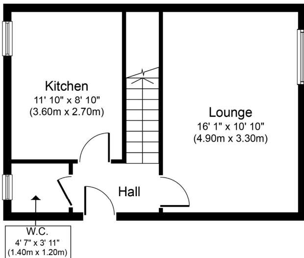
Ground Floor Approximate Floor Area 369 sq. ft. (34.3 sq. m.)
